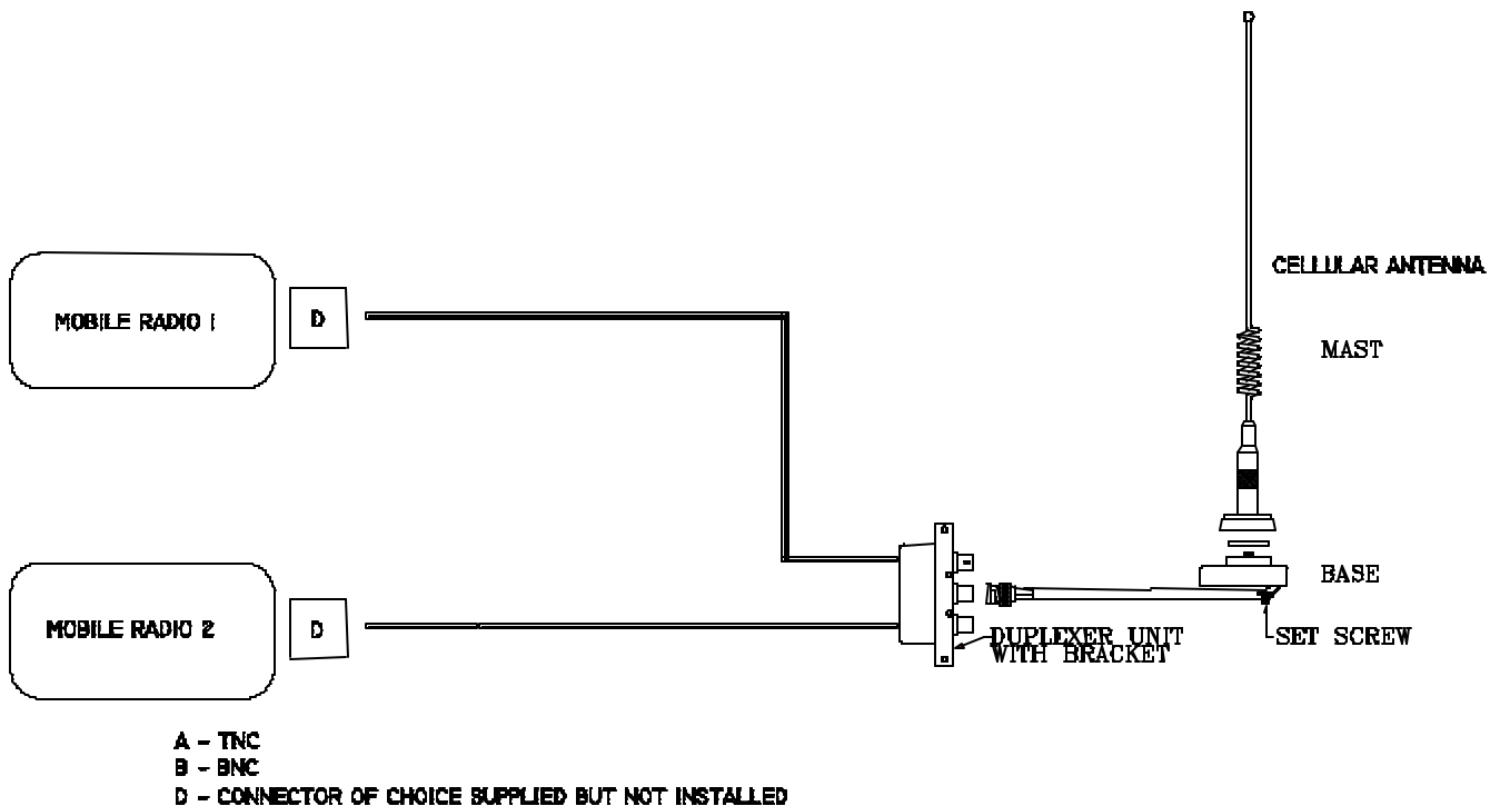
VHF/CEL Dual Band Cellular Antenna Configuration
