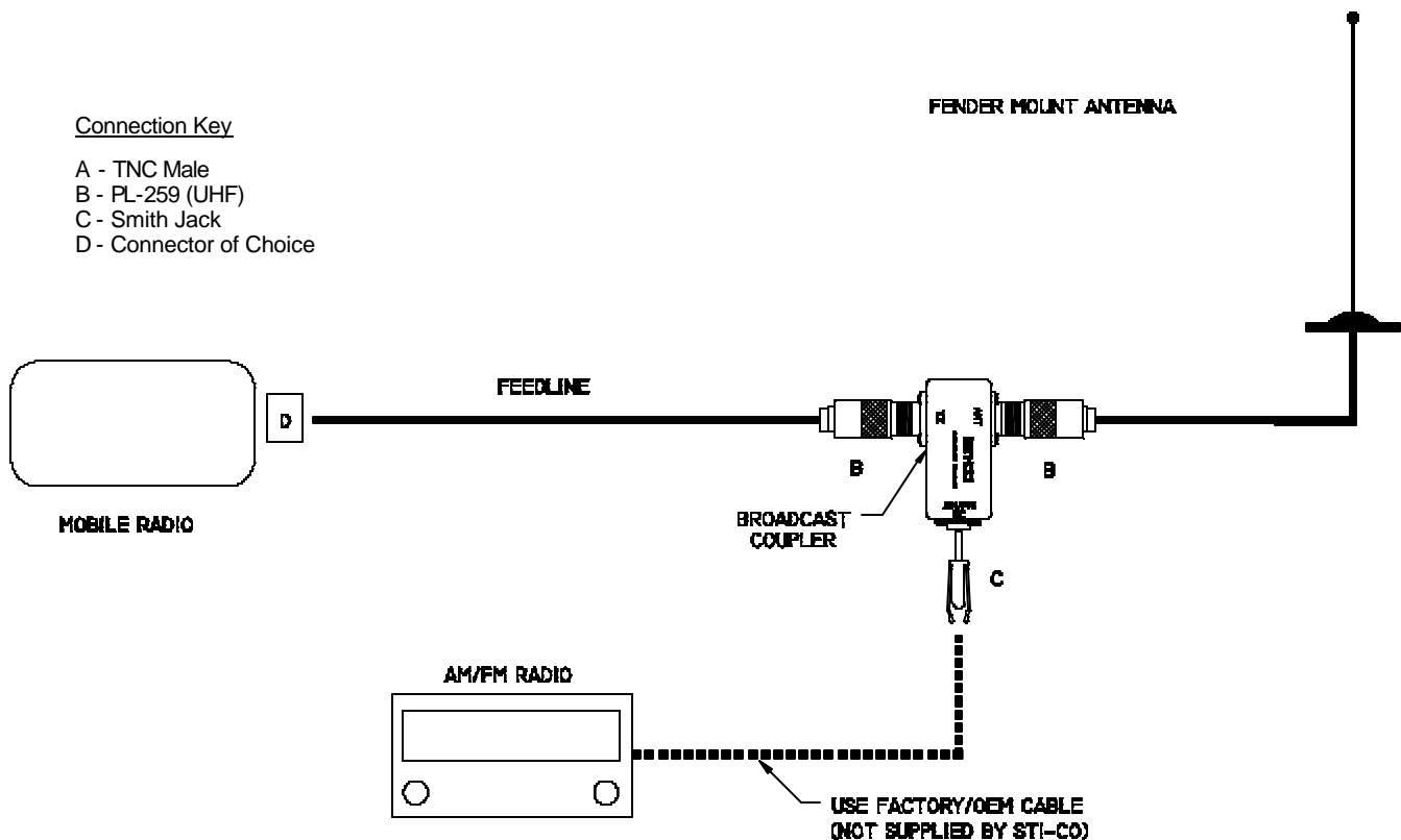
Cellular Band Fender Mount Antennas
