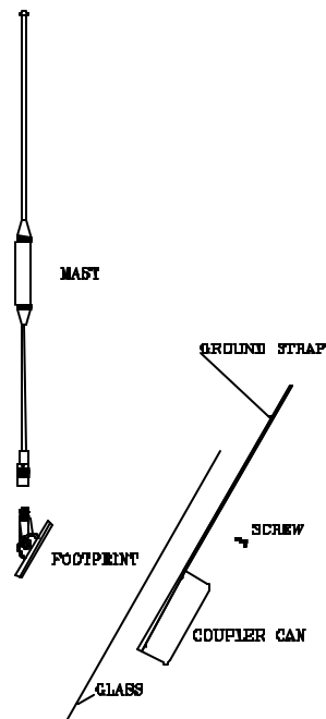
Figure 5 – General Assembly
